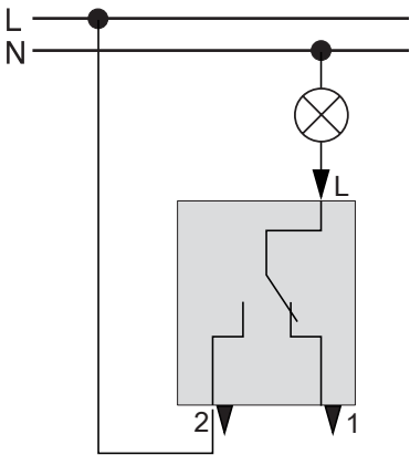
One-way/Two-way switch Mxx3x16-0000
