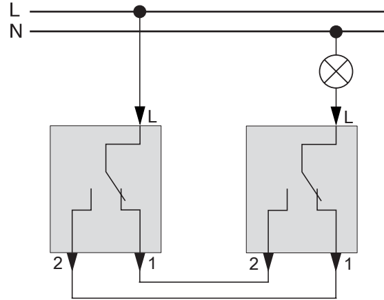
One-way/ Two-way switch Mxx3x16-0000
